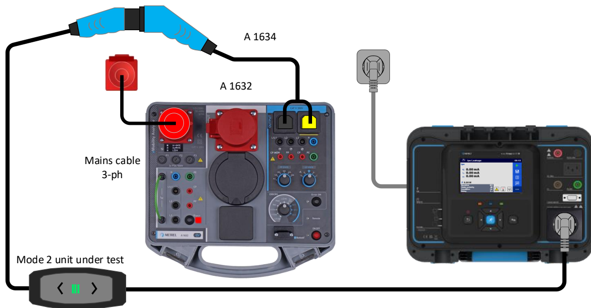
Figure 42_PE leakage current
