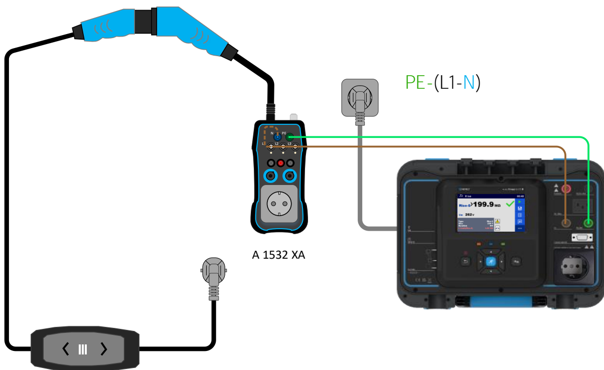
Figure 67_Insulation resistance
