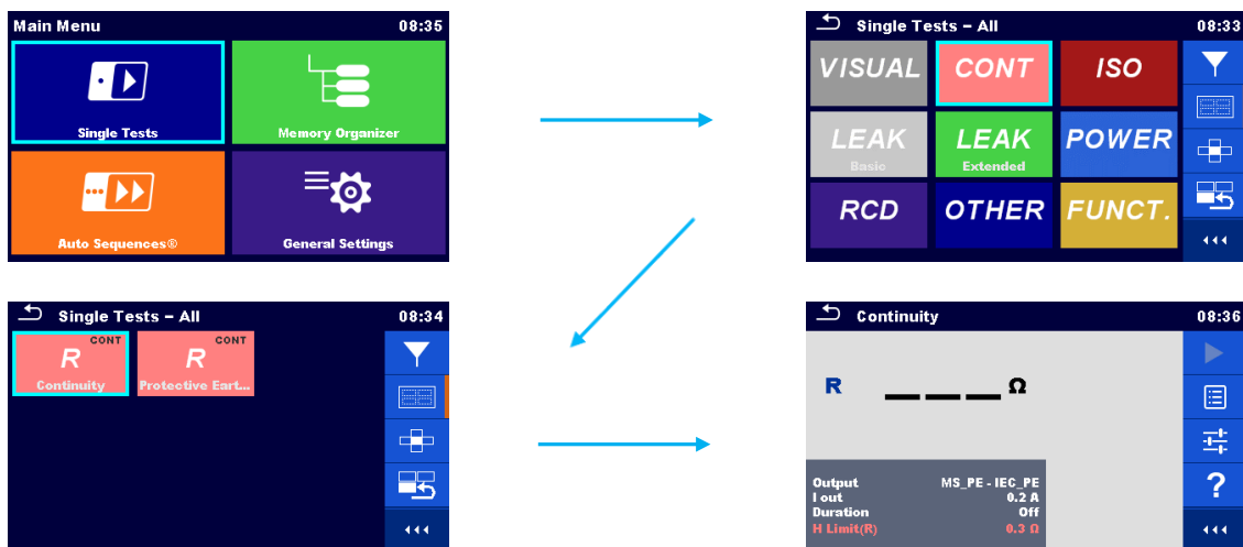
Figure 32_Earth continuity setup
