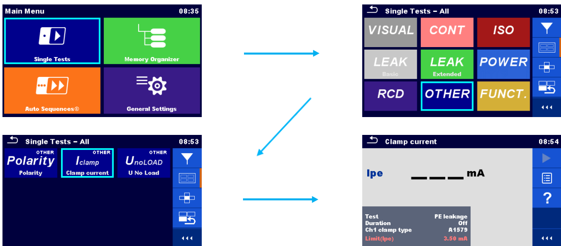
Figure 16_Current clamp setup
